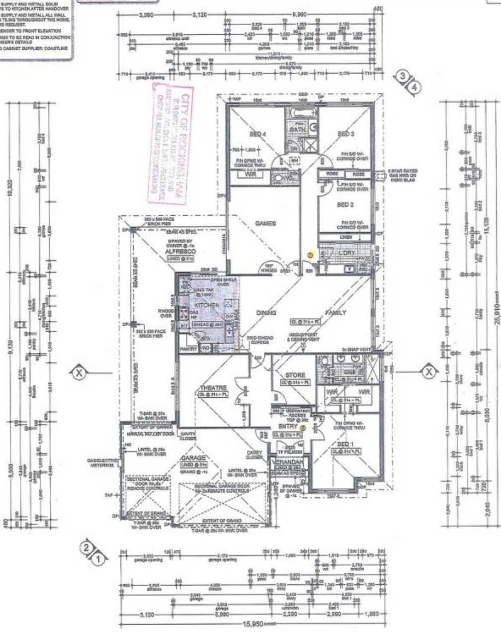
FLOOR PLAN 1:100
